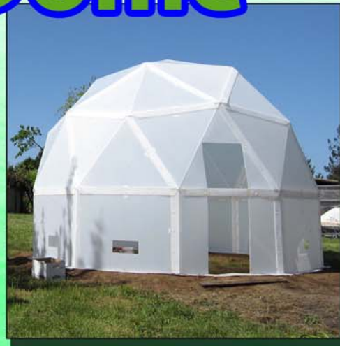
Assembled Green-Dome before installing door frame.
